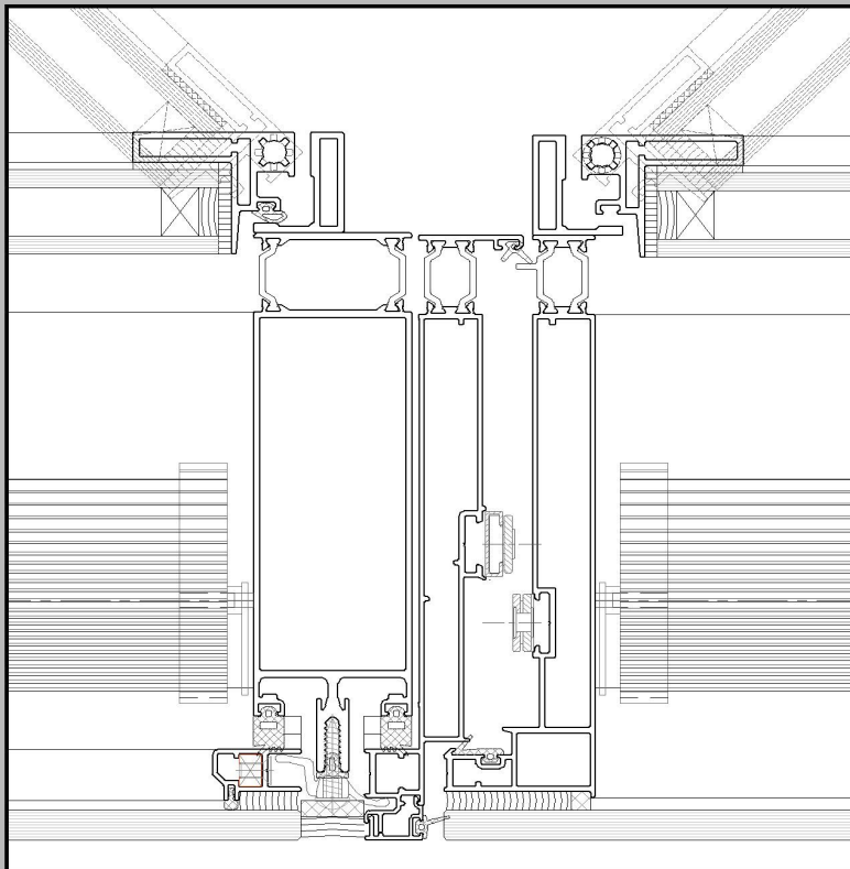
Horizontal Cut 4
