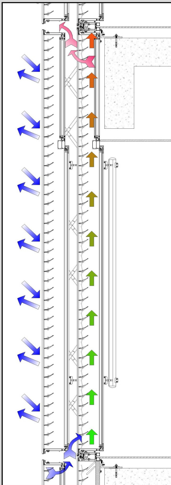
Vertical Section 2-2
