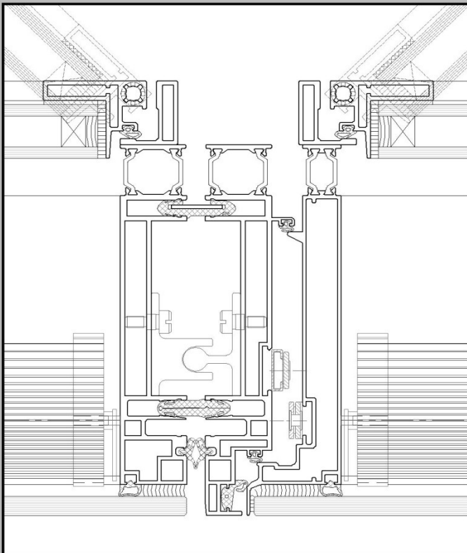
Horizontal Cut 4
