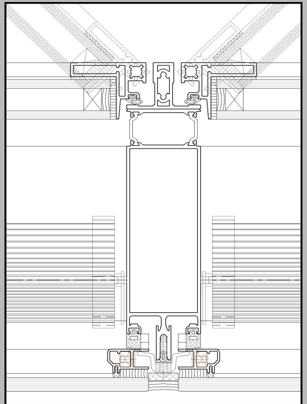
Horizontal Cut 5
