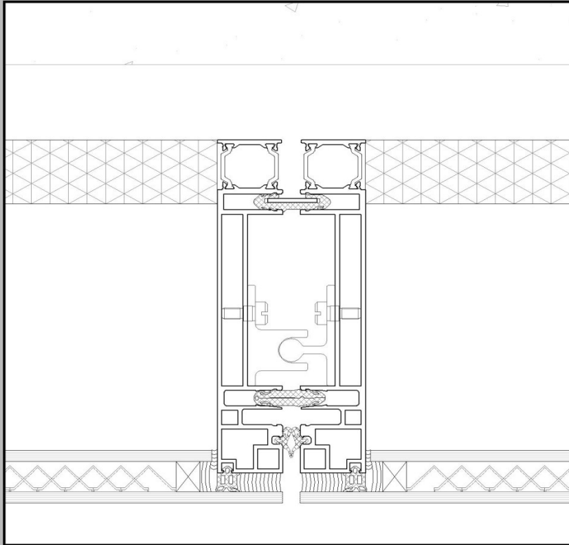
Horizontal Cut 4
