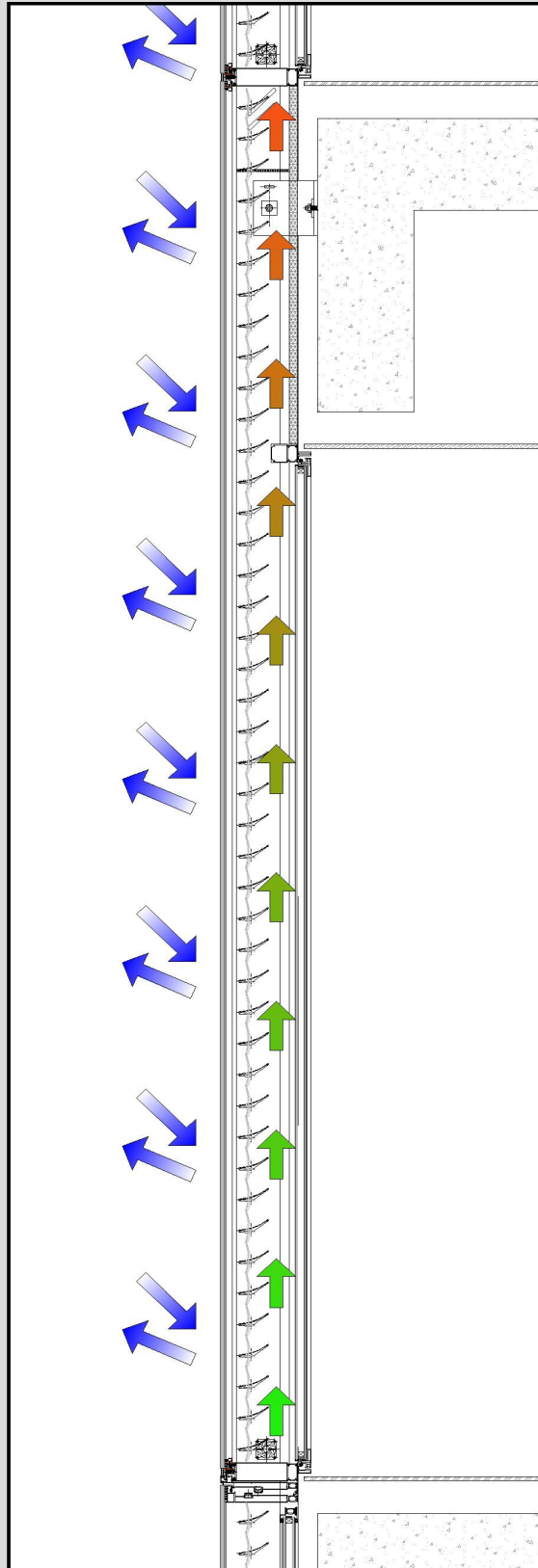
Vertical Section 1-1
