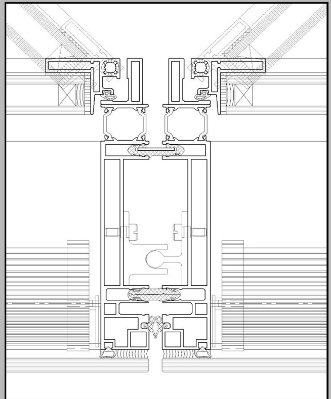
Horizontal Cut 5
