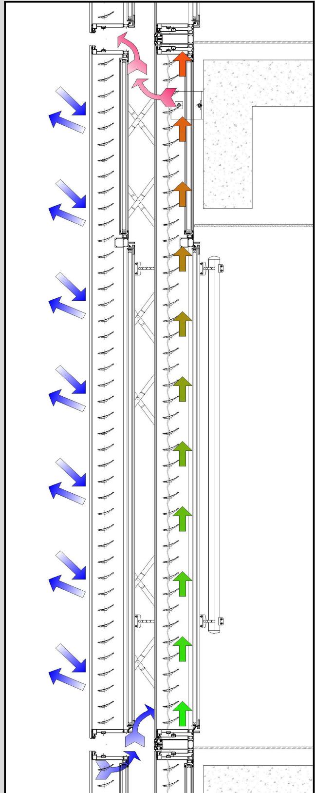
Vertical Section 2-2
