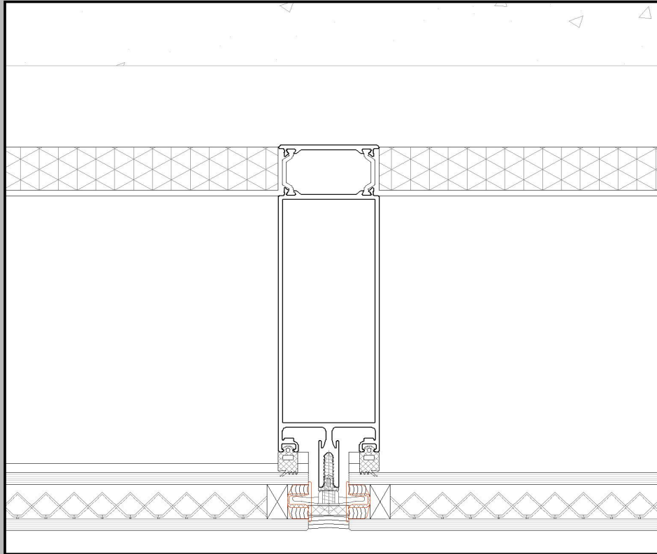
Horizontal Cut 4
